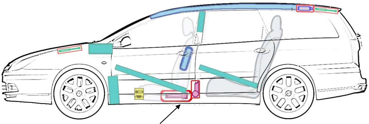
Pyrotechnic lap belt return for the front passenger only
